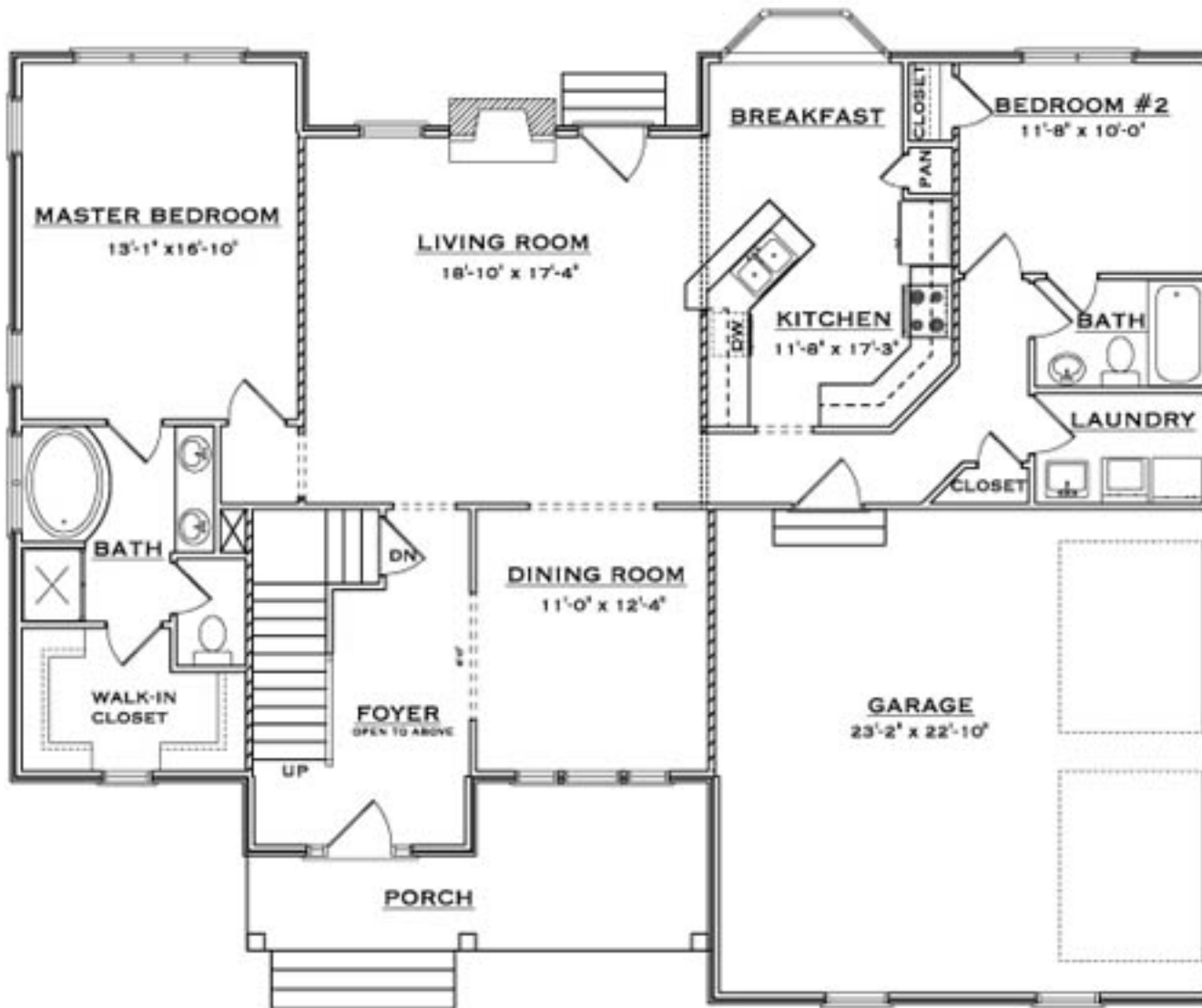
The Brookhaven FIRST FLOOR PLAN
